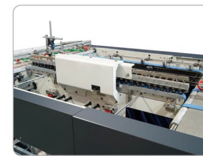
▲ Top sheet side register
