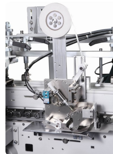
▲ Optional: Double side tape applicator
