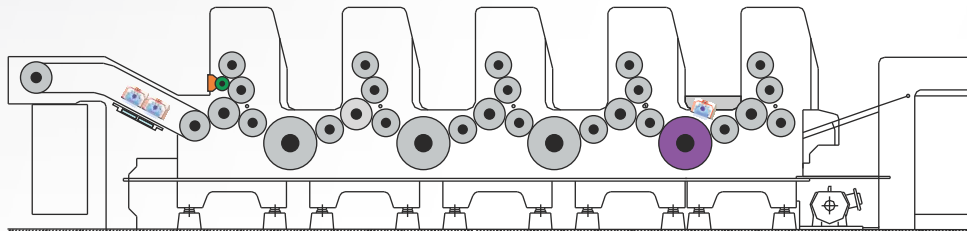
One ID + Two EOP, Configuration on a Five Color Press
