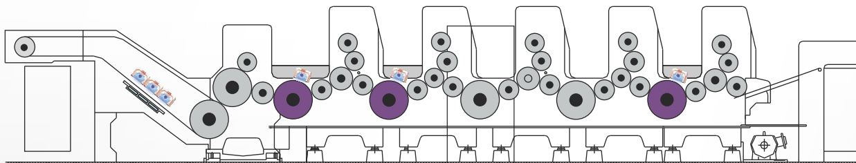
Three ID + Three EOP, Configuration on a Five Color with Coater Press
