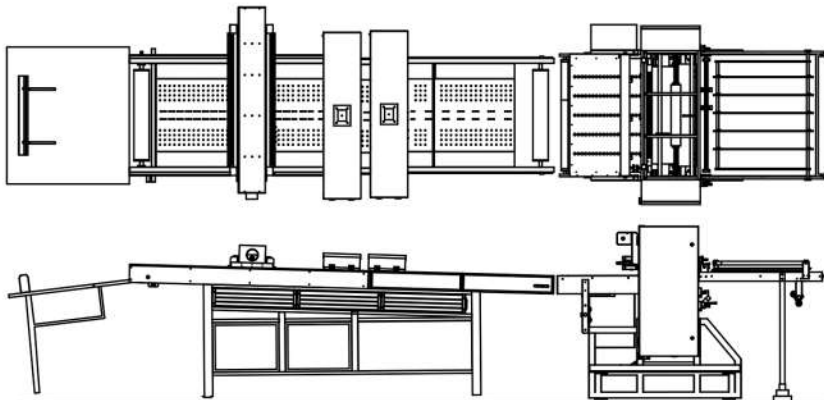
Hand-feed Roller Coater for UV/Aqueous/Primer Coatings
