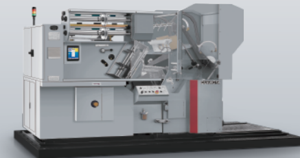
TL 780 Automatic Foil Stamping and Die Cutting Machine (longitudinal 2, transversal 2) 自动烫金模切机(两纵两横)
